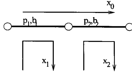
Fig. 1. Two-Link Case
